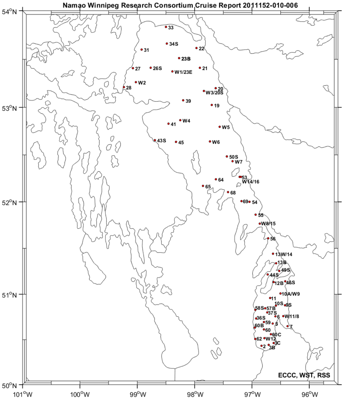
Figure 4-1. Plot of SeaBird profile stations visited during the Namao Research Consortium Cruise 2011152-010-006.
