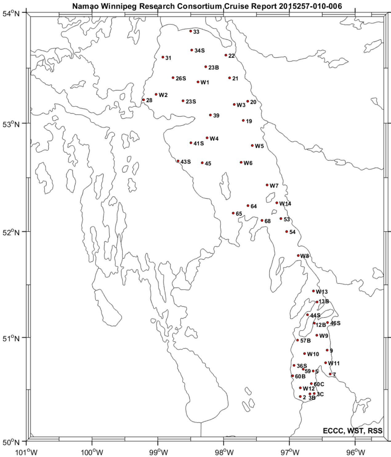
Figure 4-1. Plot of SeaBird profile stations visited during the Nainian Research Consortium Cruise 2015257-010-000.
