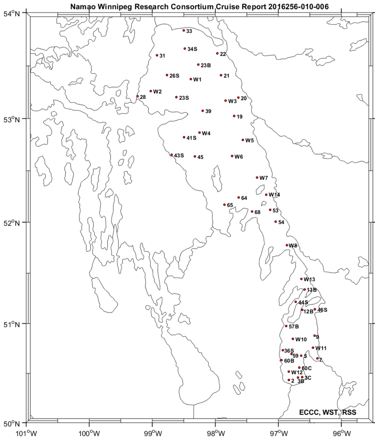
Figure 4-1. Plot of SeaBird profile stations visited during the Nainiwan Research Consortium Cruise 2016256-010-006.
